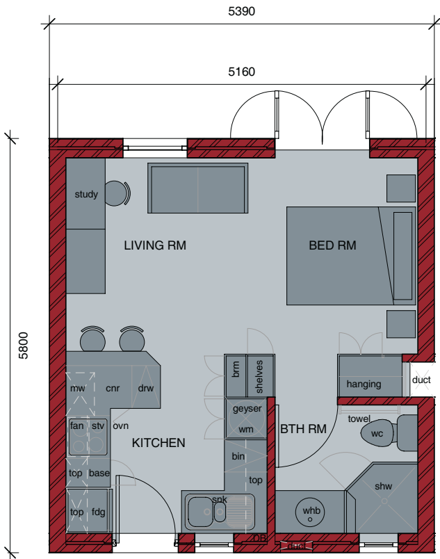
bachelor floor plan
